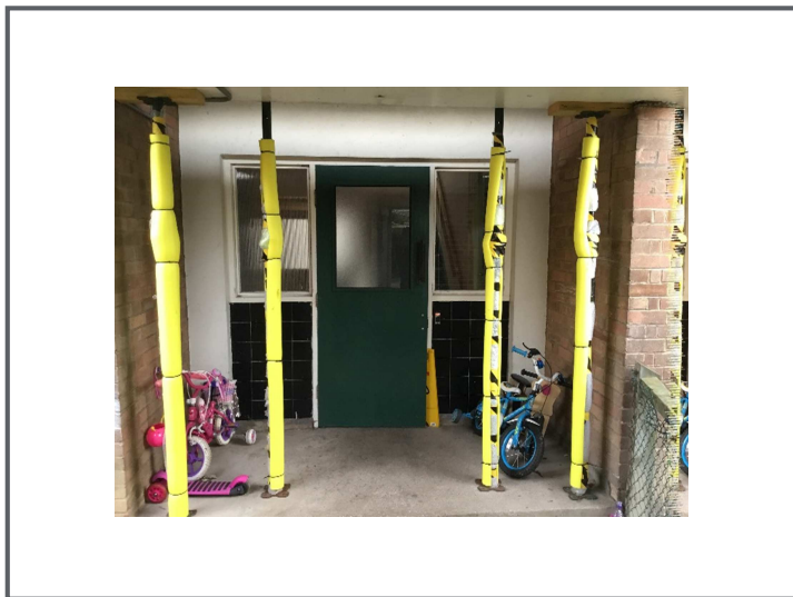
Photo 5 – Ekin Road Block Rear Door and Acrow Props
